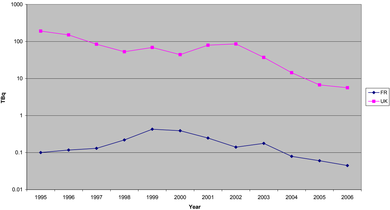
Figure 2.8: Tc-99 discharges from the nuclear fuel reprocessing sub-sector per country
